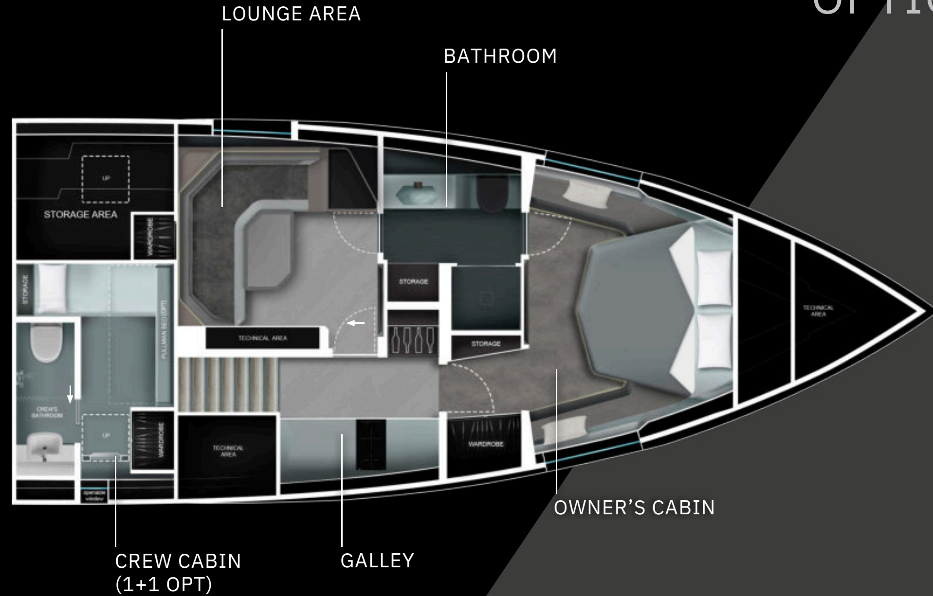
1 CABIN + 1 LOUNGE LAYOUT
