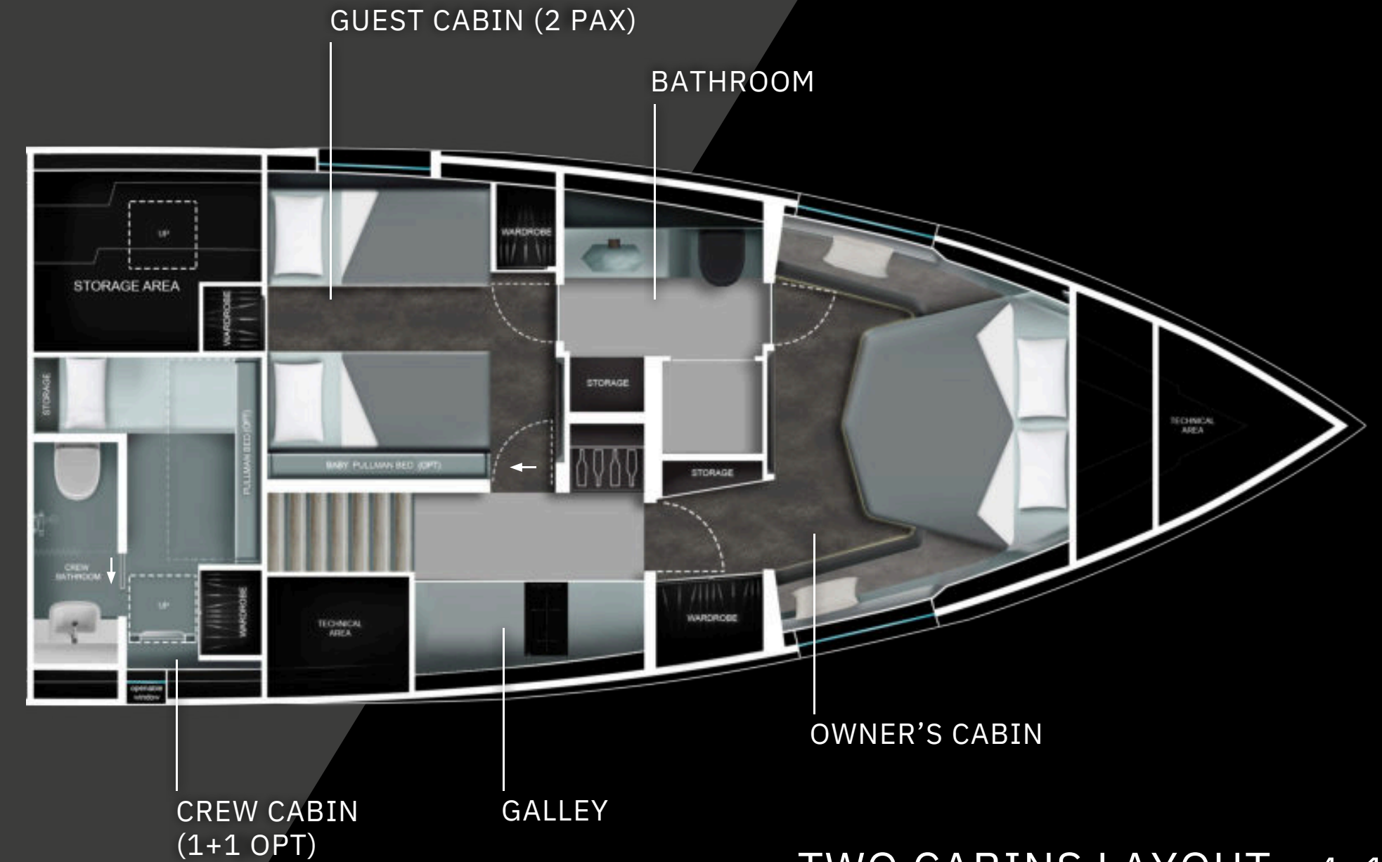
TWO CABINS LAYOUT 4+1 GUEST
